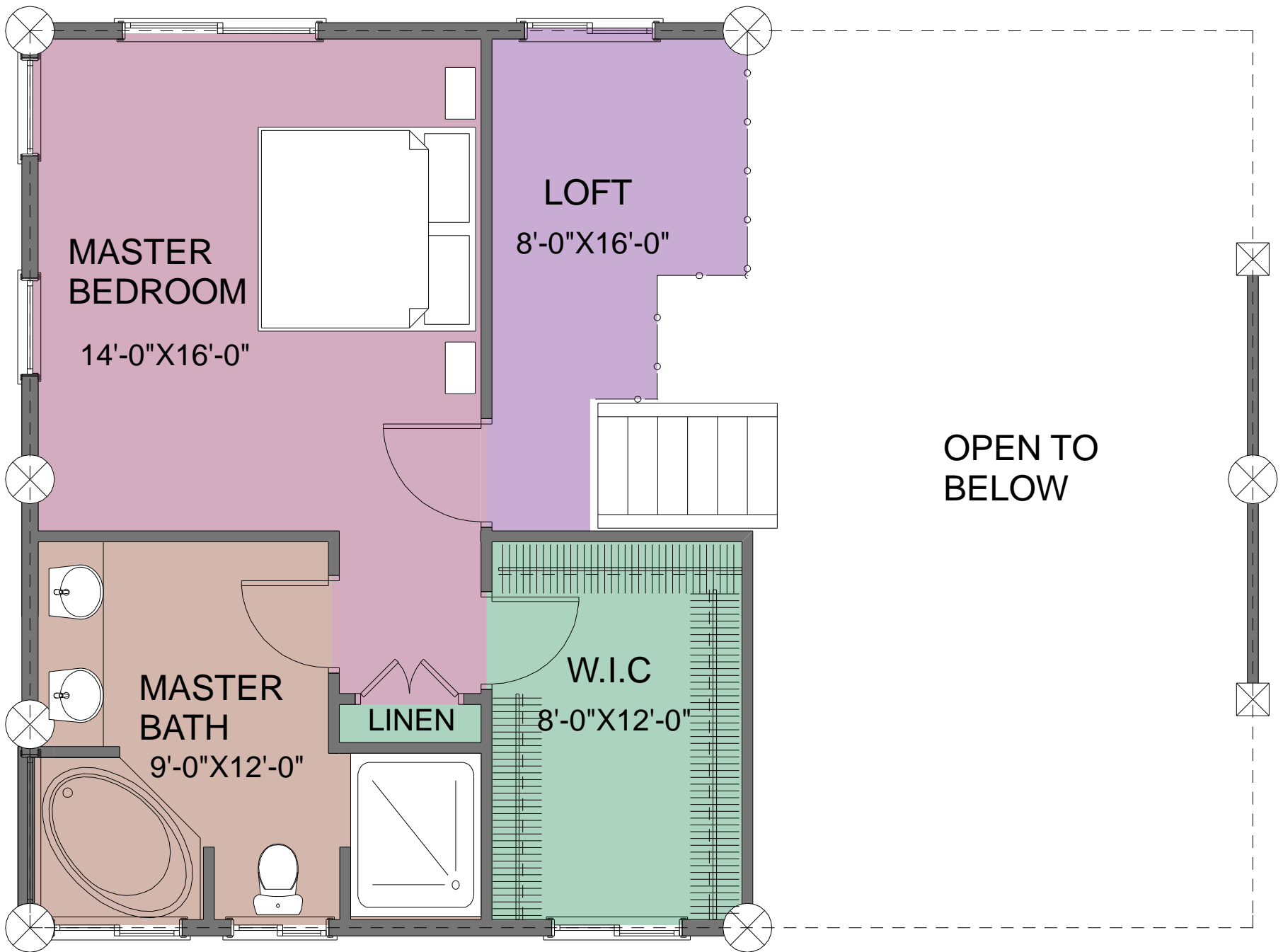
SECOND FLOOR PLAN AREA: 575 SQ. FT.
