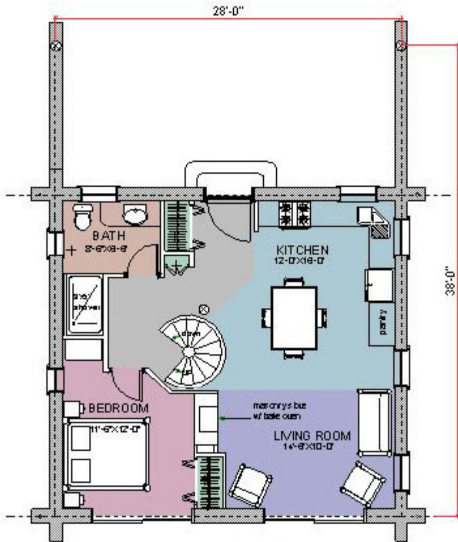
FIRST FLOOR PLAN AREA: 750 SQ. FT.
